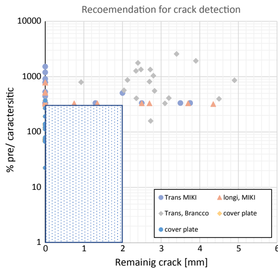
Fig 18. Ratio (\frac{prefatiguedlife}{characteristicfatiguelife}) as a function of the remaining fatigue life.
